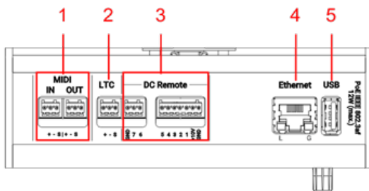
grandMA3 I/O Node DIN Rail rear panel
